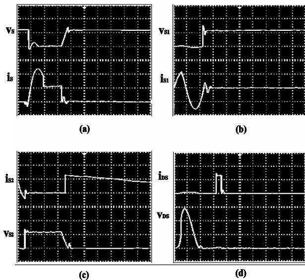
Fig. 5 Experimental voltage and current waveforms: (a) main switch S: V_S ; I_S (V: 10 V/div, I: 10 A/div, time: 0.5 \mu s/div), (b) auxiliary switch S_1 : V_{S1} ; I_{S1} (V: 10 V/div, I: 10 A/div, time: 0.5 \mu s/div), (c) synchronous switch S_2 : V_{S2} ; I_{S2} (V: 10 V/div, I: 10 A/div, time: 0.5
