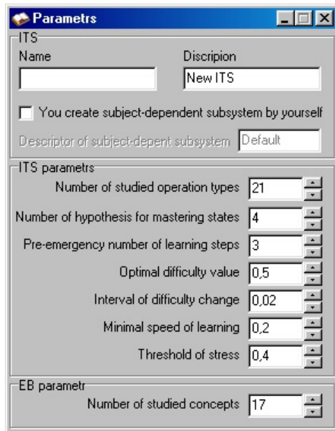
Fig. 4 Parameters of learning process model
