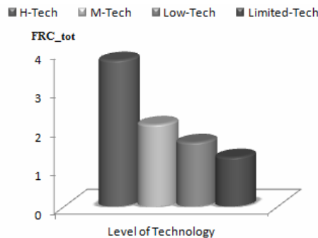
Fig. 3 Number of Total Failure Rate Categories according to “technological complexity” classification
