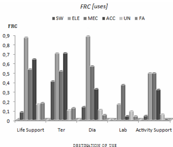
Fig. 5 Number of Failures per Category per n° of devices classified according the “destination of use” classification
