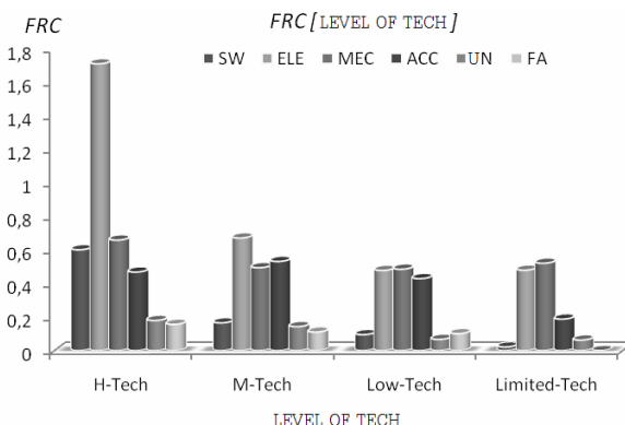
Fig. 4 Number of Failures per Category per n° of devices classified according the technological complexity classification
