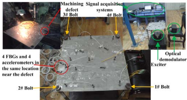
Fig. 3 Picture of the experiment
