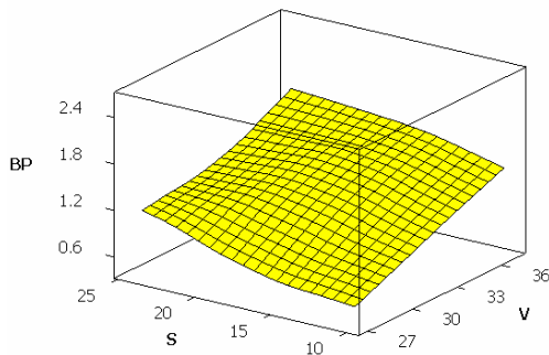
Fig. 6 The effects of welding speed and voltage on weld penetration
