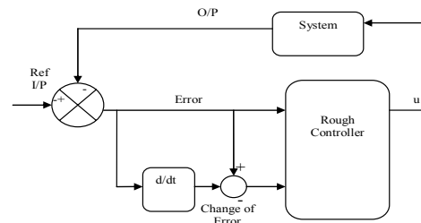
Fig. 1 Block diagram of Rough Controller For OTC
