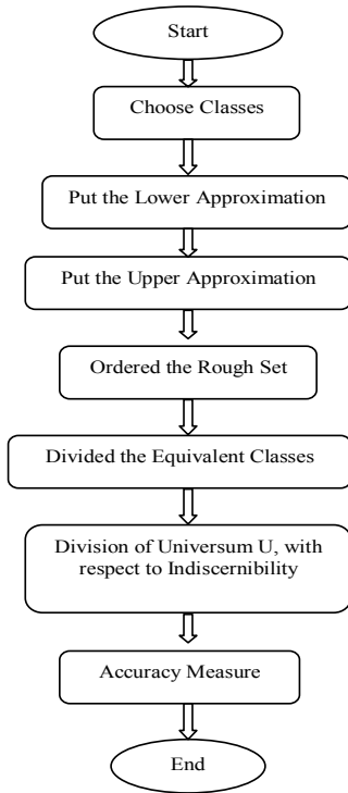
Fig. 2 The main structure of Rough Controller
