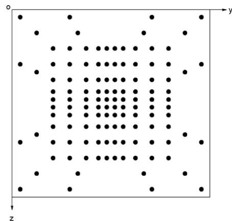
Fig. 4 Sensor distribution
