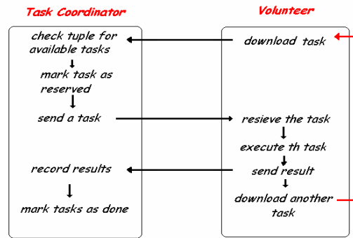
Fig. 4 Volunteer-Task-coordinator protocol
