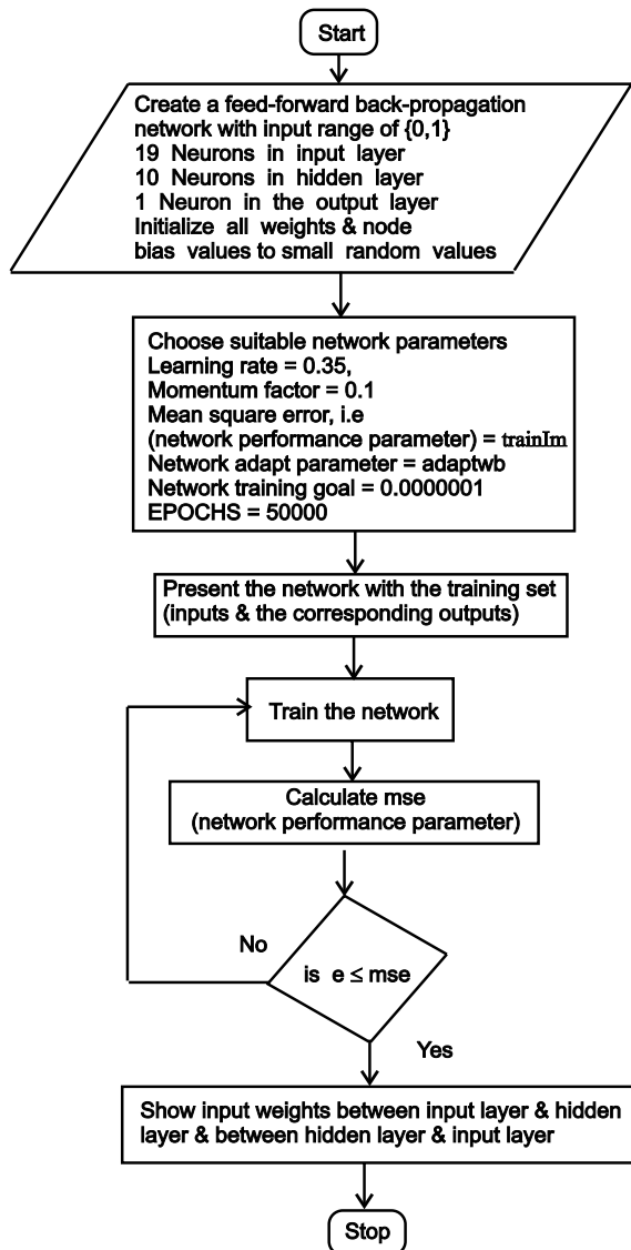
Fig. 9 Network architecture & the algorithm used
