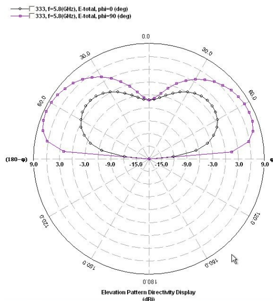
Fig. 7. Radiation pattern for geometry 1
