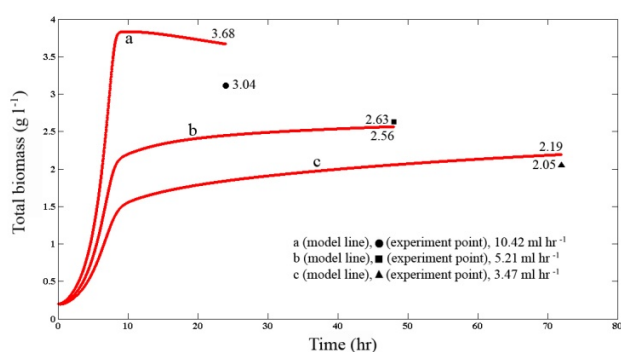
Fig. 4 Comparison between the final concentrations of experimental and predicted biomass at glycerol concentration of 60 \text{ g L}^{-1} ( C/N=10 ) and feed flow rates of 10.42 (a: ●), 5.21 (b: ■) and 3.47 (c: ▲) \text{ml hr}^{-1}
