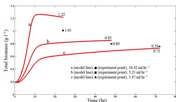
Fig. 5 Comparison between the final concentrations of experimental and predicted biomass at glycerol concentration of 20 \text{ g L}^{-1} ( C/N=10 ) and feed flow rates of 10.42 (a: ●), 5.21 (b: ■) and 3.47 (c: ▲) \text{ml hr}^{-1}
