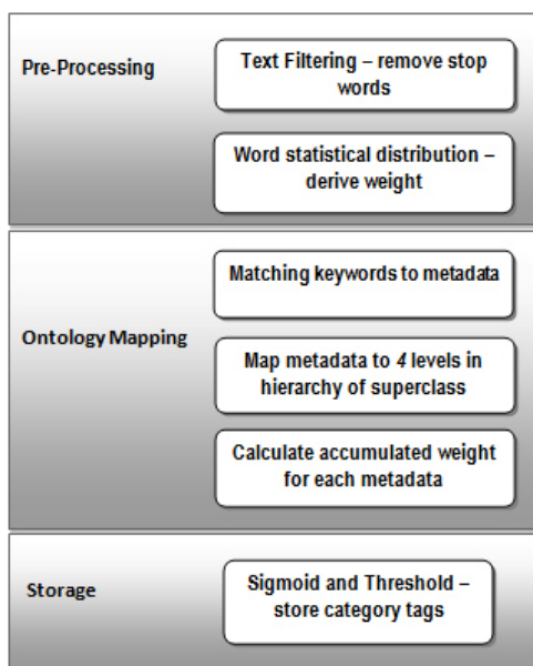
Fig. 2 Processes involved in the ontology mapping phase
