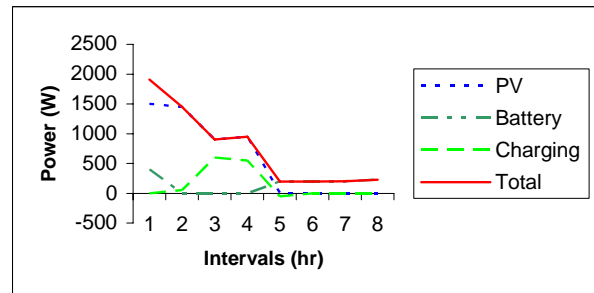
Fig. 5 The primary and secondary energy sources
