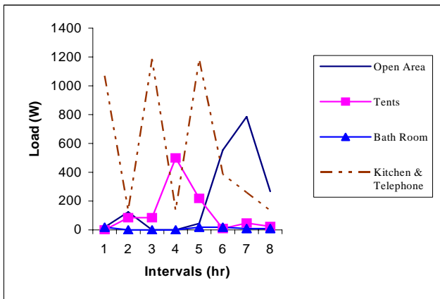
Fig. 1 Load variation of various sections
