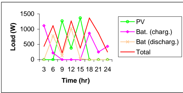
Fig. 6 The primary and secondary energy sources
