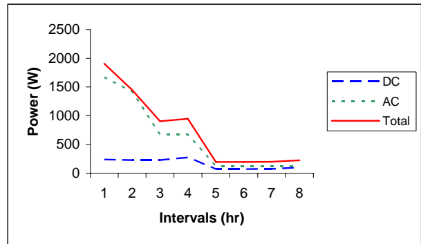
Fig. 3 The various required load
