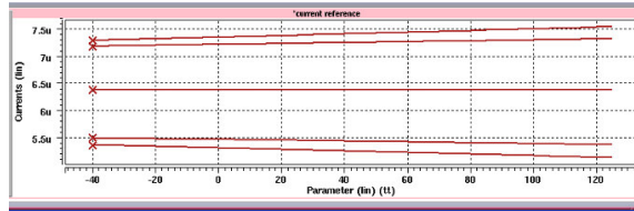
Fig. 8. Current reference under the five corner condition.
