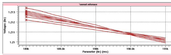
Fig. 11. Output Voltage at Varying Resistor Value With Respect to Temperature
