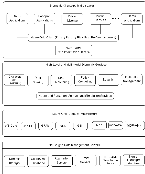
Fig. 4. Grid-based MBP-ANN framework for multimodal biometrics
