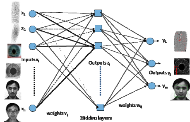
Fig. 4. MBP-ANN model for multimodal biometric fusion
