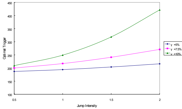
Fig. 8. The Jump Effect under a Jump Amplitude Process
