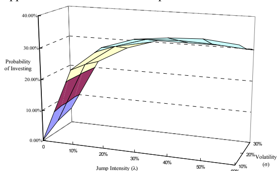
Fig. 4. The Probability of Investing as a Function of Jump Intensity ( \lambda ) Given an MX Process
