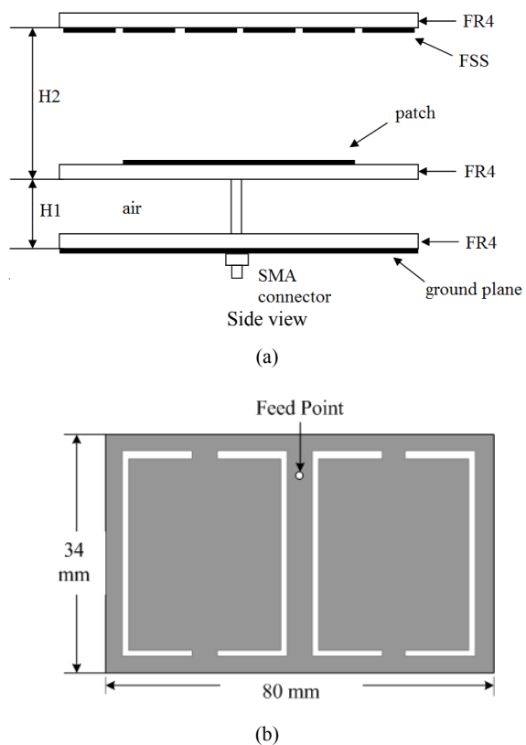
Fig. 1 (a) The proposed antenna geometry and (b) U-slotted patch antenna
