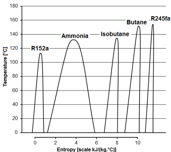
Fig. 4 Saturation vapor regions of the working fluids: R152a, Ammonia, Isobutane, Butane and R245fa
