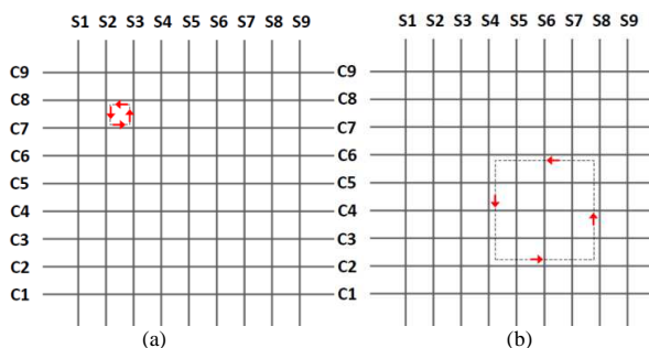
Fig. 4 The proposed coil system can generate circular coils for different sizes. (a). A small circular coil is configured by controlling the currents in wires of S2-S3-C7-C8. (b). A large circular coil is configured by controlling the currents in wires of S4-S8-C2-C6
