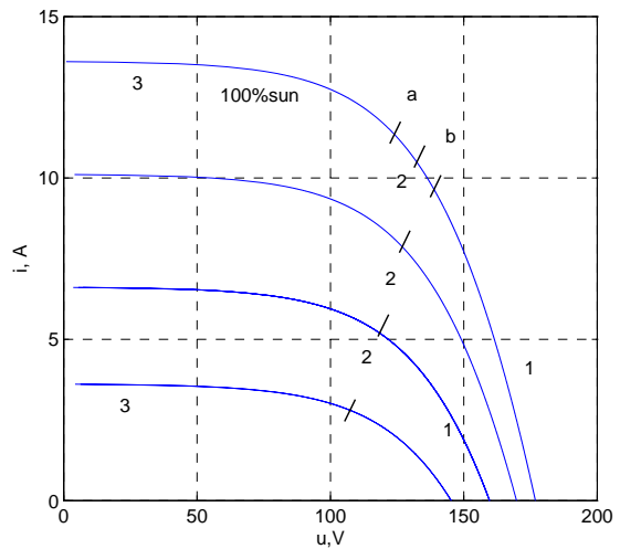
Fig. 5. The typical parts of the calculated family of the I - V characteristic with different values of insulation or SC current: 1-characteristic of the voltage source with a high internal resistance, 2- maximum load power point, 3- characteristic of the current source
