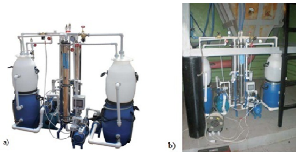
Fig. 12 Membrane pilot plant for wastewater treatment and concentrate utilization: a) 300 liter per hour membrane pilot plant; b) pilot testing at municipal wastewater facilities
