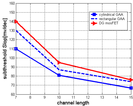
Fig. 6 Subthreshold swing as a function of channel length for rectangular and cylindrical SNWTs and DG MOSFET
