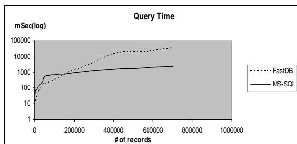
Fig. 2 Comparison of selection time between FastDB and MS-SQL for varying number of records
