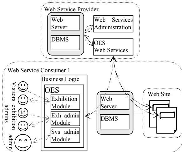
Fig. 2 The OES Web Services Architecture
