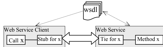
Fig. 3 The JAX-RPC Architecture
