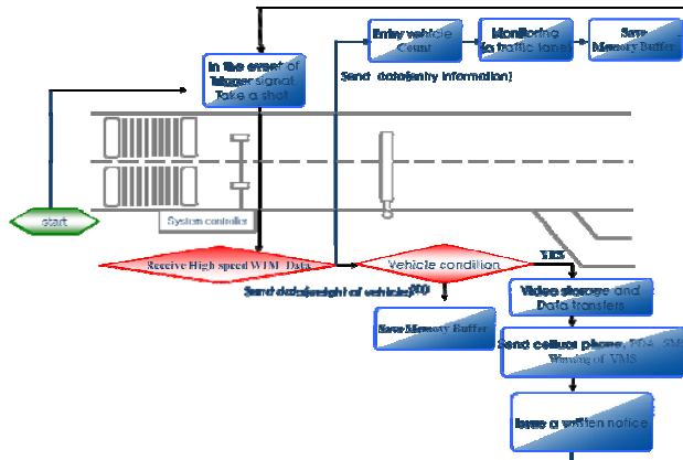
Fig. 4 System algorithm
