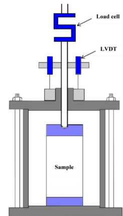
Fig. 1 The schematic of a typical repeated load triaxial test apparatus (modified from [4])
