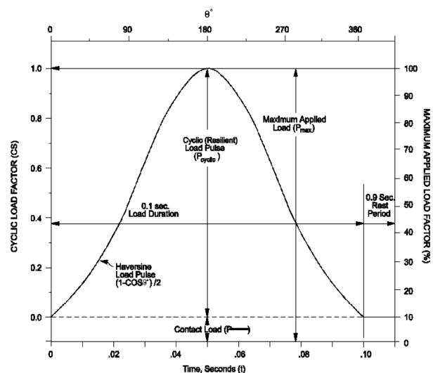
Fig. 4 The loading cycle waveform ([20])
