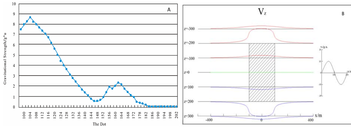
Fig. 2 The tunnel gravity measurement of three dimensional unusual Significance: A. The gravitational strength of the dot. B. The sketch of the tunnel gravity measurement of three dimensional unusual significance
