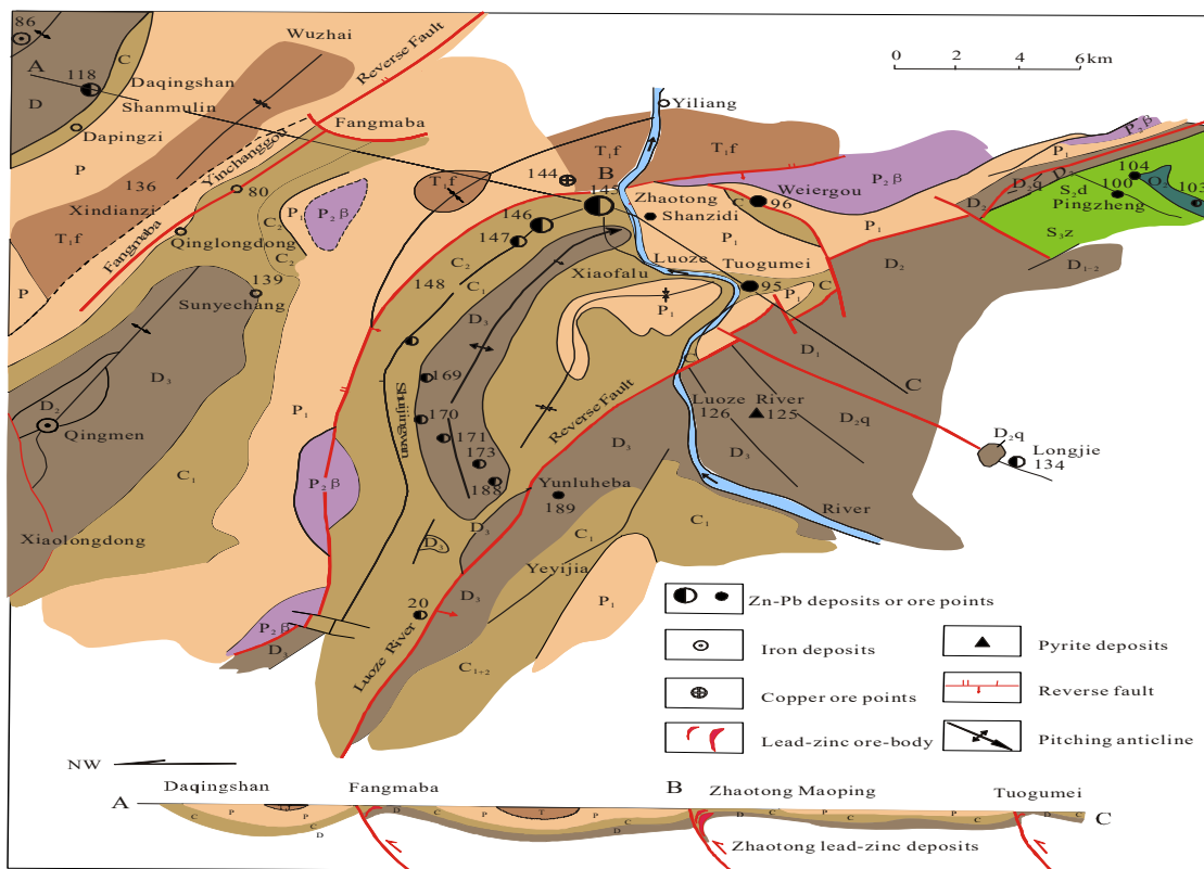
Fig. 1 Simplified geological map of the Zhaotong Maoping Zn–Pb–(Ag–Ge) ore district [9]
