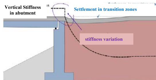
Fig. 1 Stiffness problems
