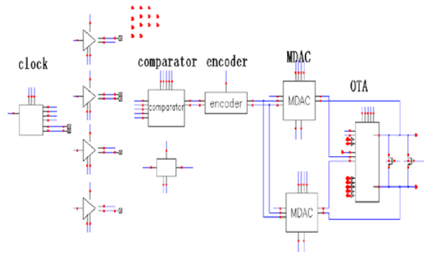
Fig. 10 The schematic of the whole stage 3.5-bit
