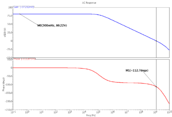
Fig. 9 AC response
