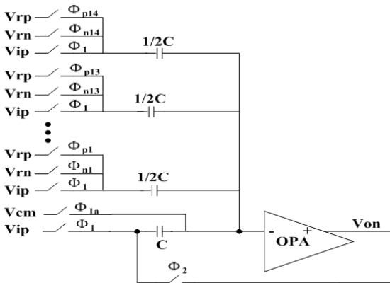
Fig. 3 Stage 3.5 bit MDAC circuit
