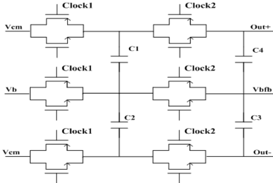
Fig. 8 Common-mode feedback with switched-capacitor
