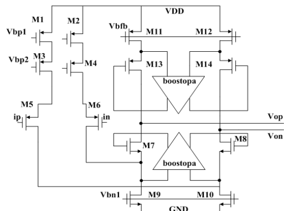
Fig. 6 The main form of the amplifier
