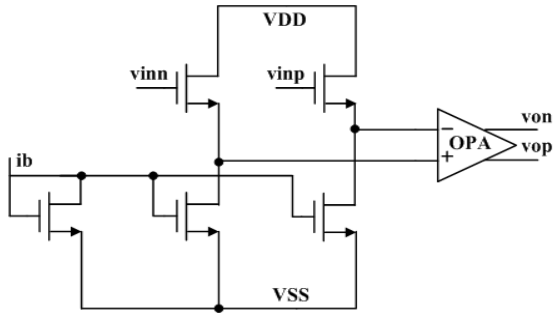
Fig. 7 The structure of the OTA
