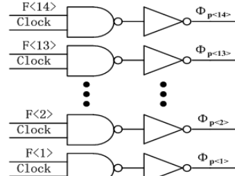
Fig. 5 The encoder circuit
