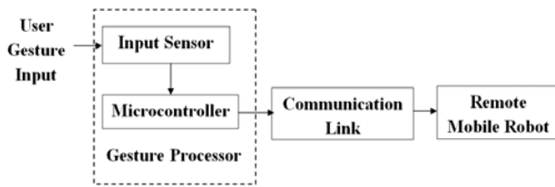
Fig. 3 System block diagram
