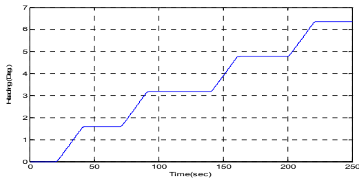
Fig. 7 Heading angle of the reference trajectory
