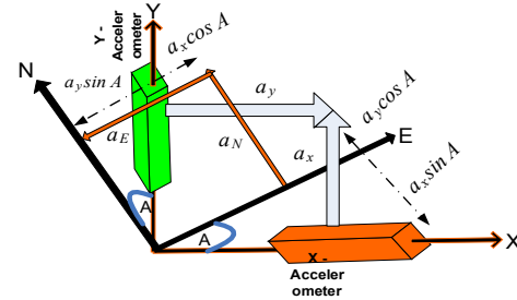
Fig. 2 Two Dimensional vector representation of transformation matrix [4]
