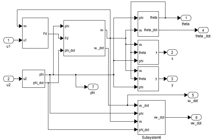
Fig. 4 Modeling Of a Car like robot Using Simulink
