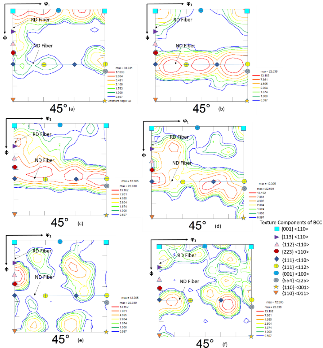
Fig. 2 (a) \phi_2 = 45^\circ sections of ODFs of cold-rolled 90%, and (b)-(f) \phi_2 = 45^\circ sections of ODFs of annealed in the range of 800 °C to 1400 °C temperatures, (b) 800 °C, (c) 850 °C, (d) 1000 °C, (e) 1250 °C, and (f) 1400 °C for 1 h
