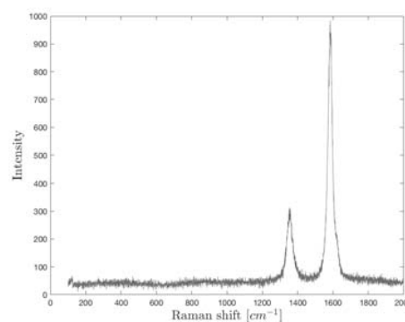
Fig. 7 The experimental outcome for the first sensor based on GO under vacuum chamber
