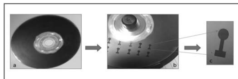
Fig. 2 Images of the final design for the first sensor: (a) GO coated substrate film stuck on a DVD disc; (b) Interdigitated capacitor sensors imprinted by LightScribe onto the GO; (c) Magnified image of an Interdigitated capacitor sensor formed by ten parallel electrodes
