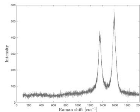
Fig. 6 The experimental outcome for the first sensor based on GO under vacuum chamber
