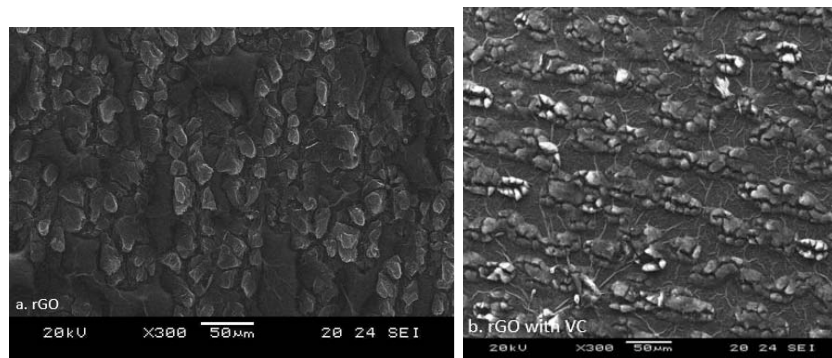
Fig. 5 Microstructural details (SEM) of rGO before and after vacuum chamber (VC)
