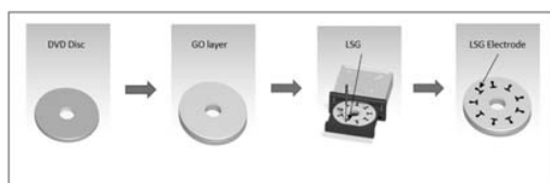
Fig. 1 The overall process of patterning LSG electrodes
