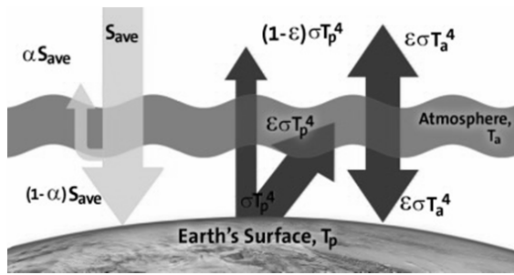
Fig. 1 Single Layer Atmospheric Model
