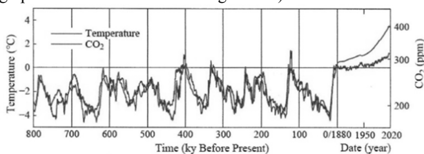
Fig. 3 Atmospheric \text{CO}_2 and global surface temperature versus time
