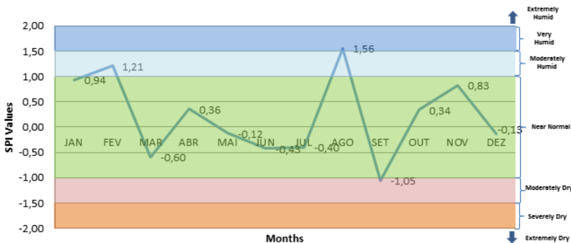
Fig. 5 SPI for Pluviometric Station 24 (2026-2100).
