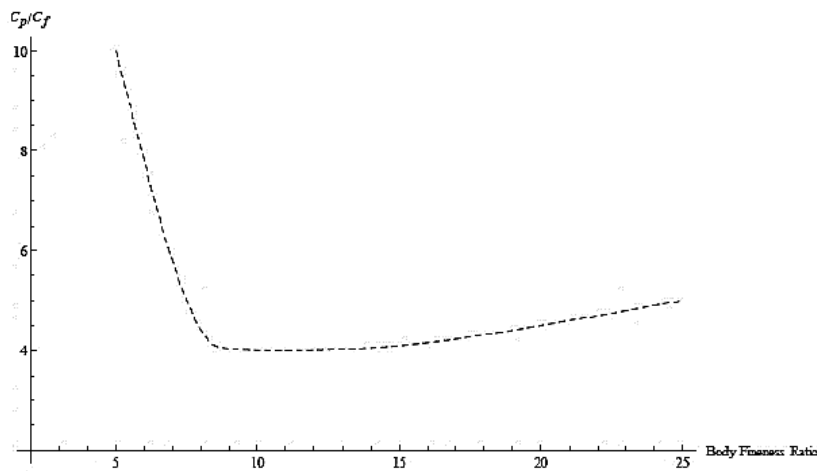
Fig. 4 Variation of drag coefficients with respect to body fineness ratio [15]
