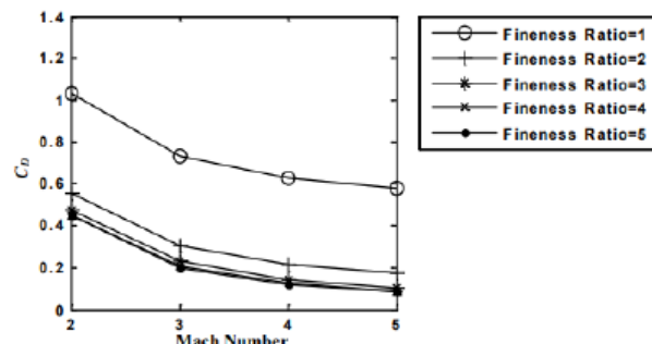
Fig. 6 Variation of drag coefficients with respect to nose cone fineness ratio [17]
