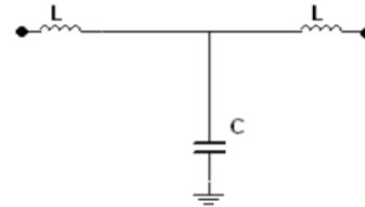
Fig. 2 Equivalent model
