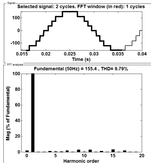
Fig. 12 FFT spectrum of CMLI output voltage at unequal DC sources (dc variation = 4.47 volts)
