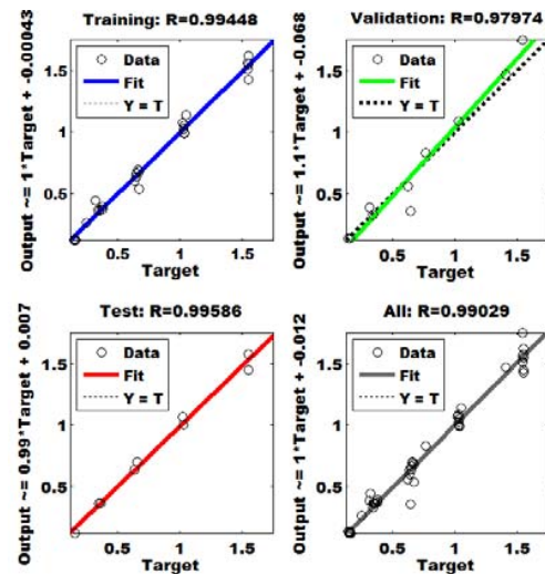
Fig. 5 ANN training regression
