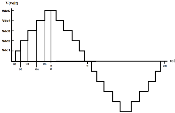
Fig. 1 Output waveform for balanced DC source
