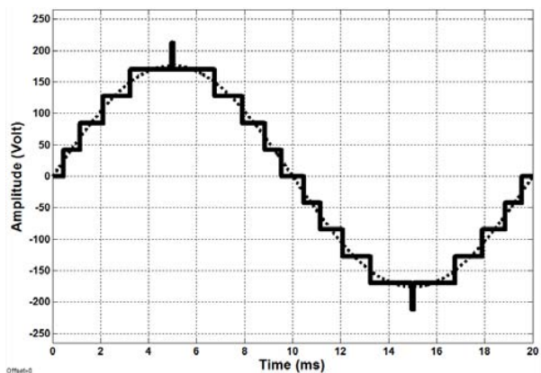
Fig. 8 The output voltage of the CMLI at equal dc sources
