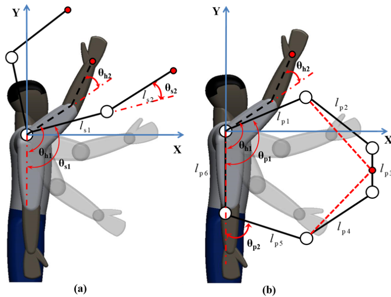
Fig. 9 (a) The simplified configuration of series mode, (b) the simplified configuration of parallel mode
