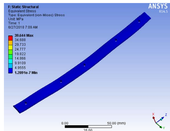
Fig. 5 (c) Von-Mises stress distribution in implant
