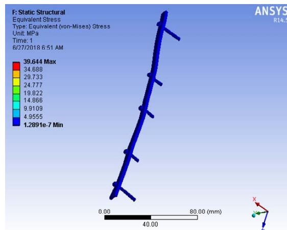
Fig. 5 (b) Von-Mises stress distribution in implant and screws
