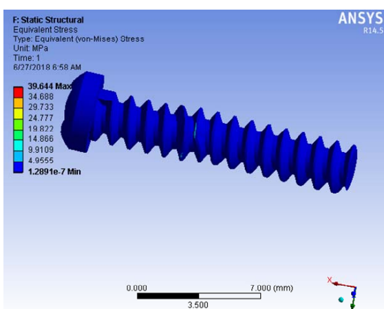
Fig. 5 (e) Von-Mises stress distribution in critical screw
