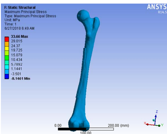
Fig. 6 (a) Maximum principal stress in clinical setup
