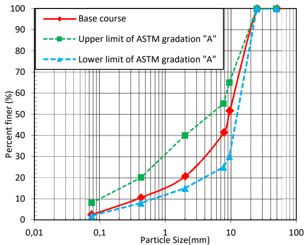
Fig. 6 Grain size distribution of base course material
