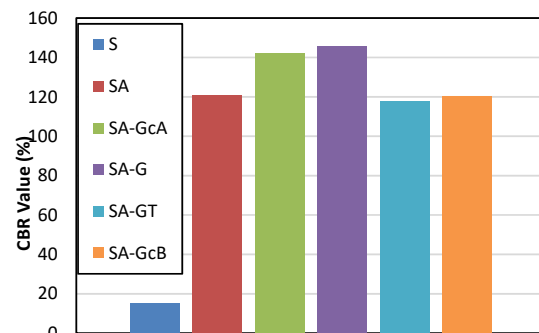
Fig. 16 Overview of the CBR values obtained from the tests
