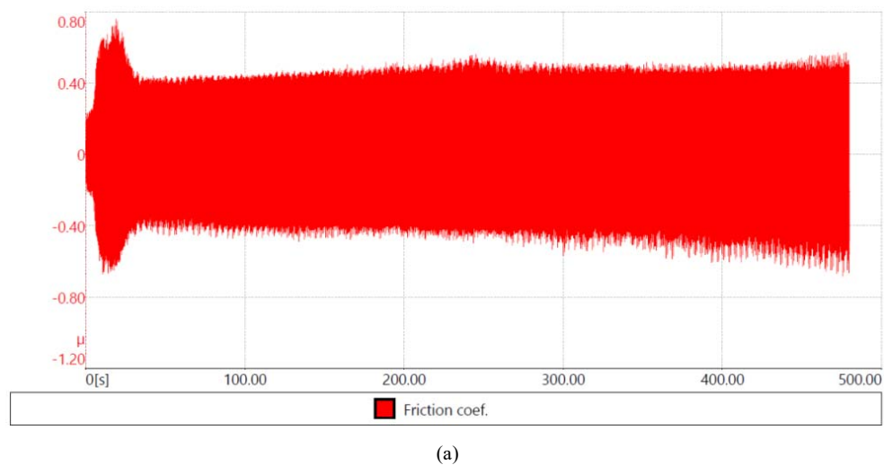
Fig. 4 Scratch test of DLC film
