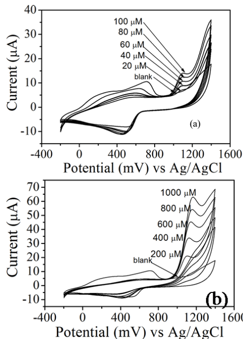
Fig. 11 CV responses of GR-PANI|GCE sensor to anthracene at 50 \text{mV s}^{-1} . Experimental conditions: 0.1 M \text{LiClO}_4 in acetonitrile/water (80:20 v/v) for (a) 20-100 \mu\text{M} and (b) 200-1000 \mu\text{M} anthracene
