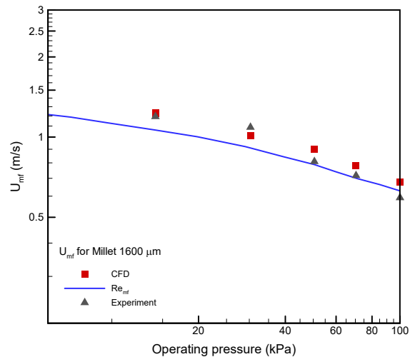
Fig. 2 Minimum fluidization velocity at reduced pressure
