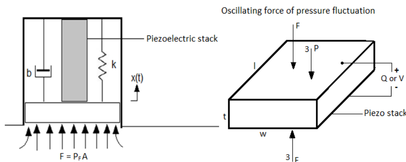
Fig. 1 Schematic diagram of the piezoelectric energy harvesting system
