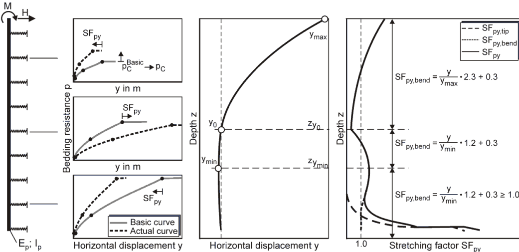
Fig. 3 Conception of the p-y approach of [7]
