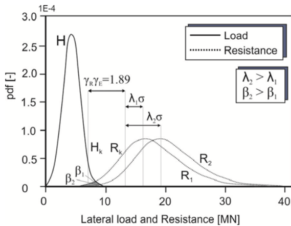
Fig. 7 Load and resistance distribution with safety factor
