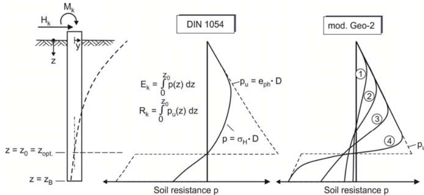
Fig. 4 ULS proof acc. to DIN 1054 and modified Geo-2 proof
