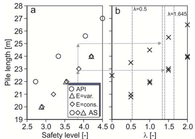
Fig. 6 Safety level (a) and \lambda -value (b) for the reference system for the ULS according to [7] and [10]
