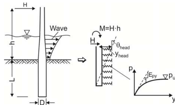
Fig. 1 Concept of p-y curves
