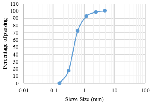
Fig. 1 Sieve Analysis of Fine Aggregate
