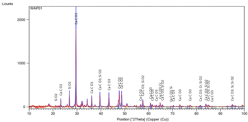
Fig. 3 XRD pattern of wood ash particles
