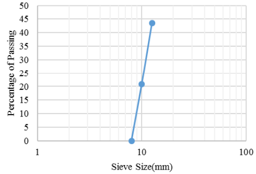
Fig. 2 Sieve Analysis of Coarse Aggregate
