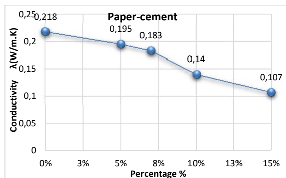
Fig. 3 Evolution of the thermal conductivity paper-cement
