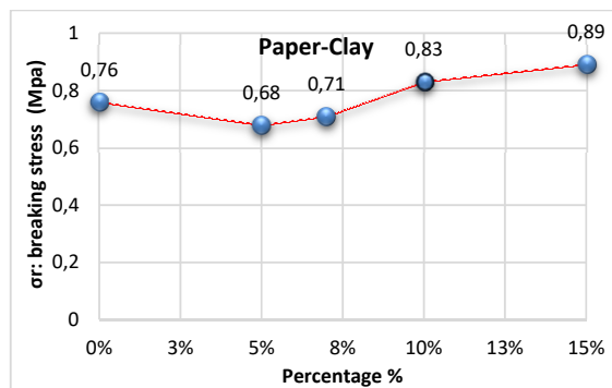
Fig. 5 Evolution of the mechanical properties of the specimens Paper-Clay (σr: breaking stress)
