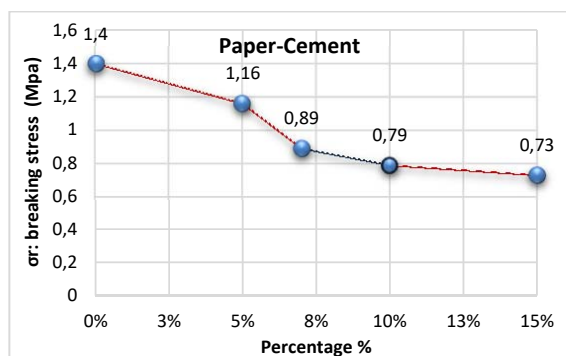
Fig. 4 Evolution of the mechanical properties of the specimens: paper-cement (σr: breaking stress)
