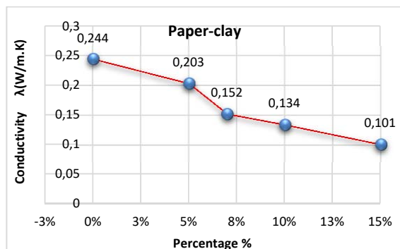
Fig. 2 Evolution of the thermal conductivity of paper-clay
