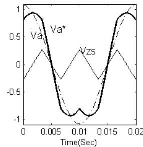
Fig. 2 Sin signal ( V_a ), zero sequence signal ( V_{zs} ) and Modulating signal ( V_a^* ): CSVPWM algorithm
