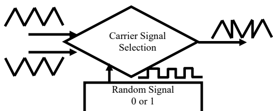
Fig. 4 Block diagram describing the basic principle of carrier selection.
