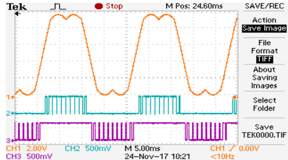
Fig. 19 RCPWM: Modulating Signal, Pulses for Inverter-I & II
