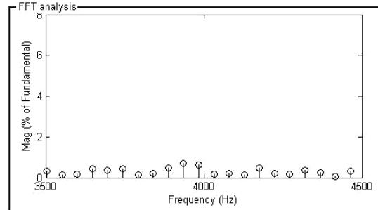
Fig. 42 RMCPWM: Zoomed Portions at and around 4 kHz
