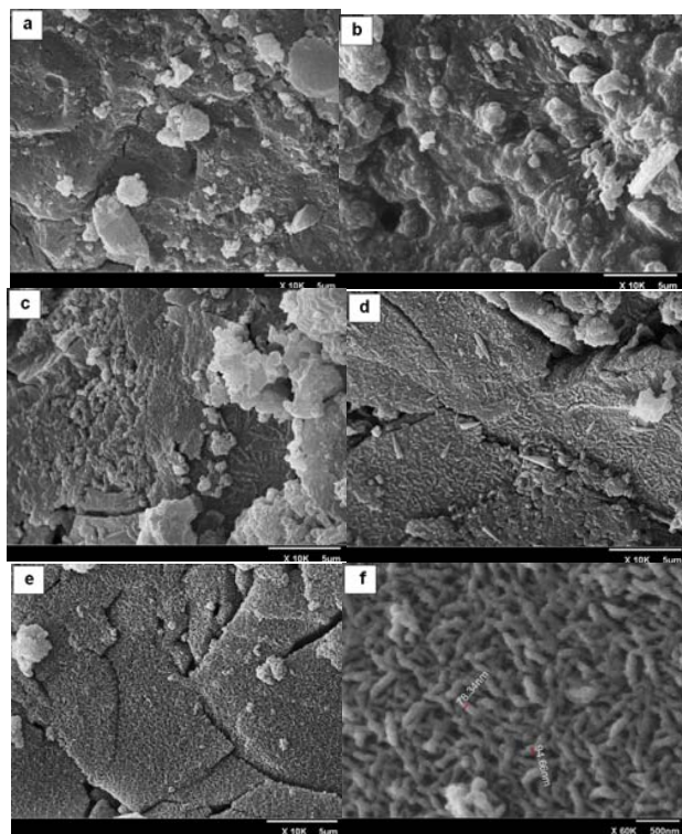
Fig. 6 SEM images of BG-5/5 before (a) and after soaking in the SBF solution for 1 (b), 3 (c), 7 (d) and 14 (e) days at magnification 10K×; and image (e) at 60K× magnification (f)
